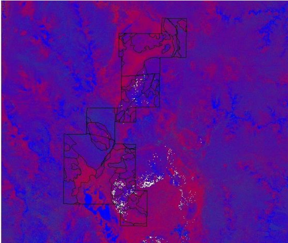
Figure 1 Estimated Fractional Cover Map
