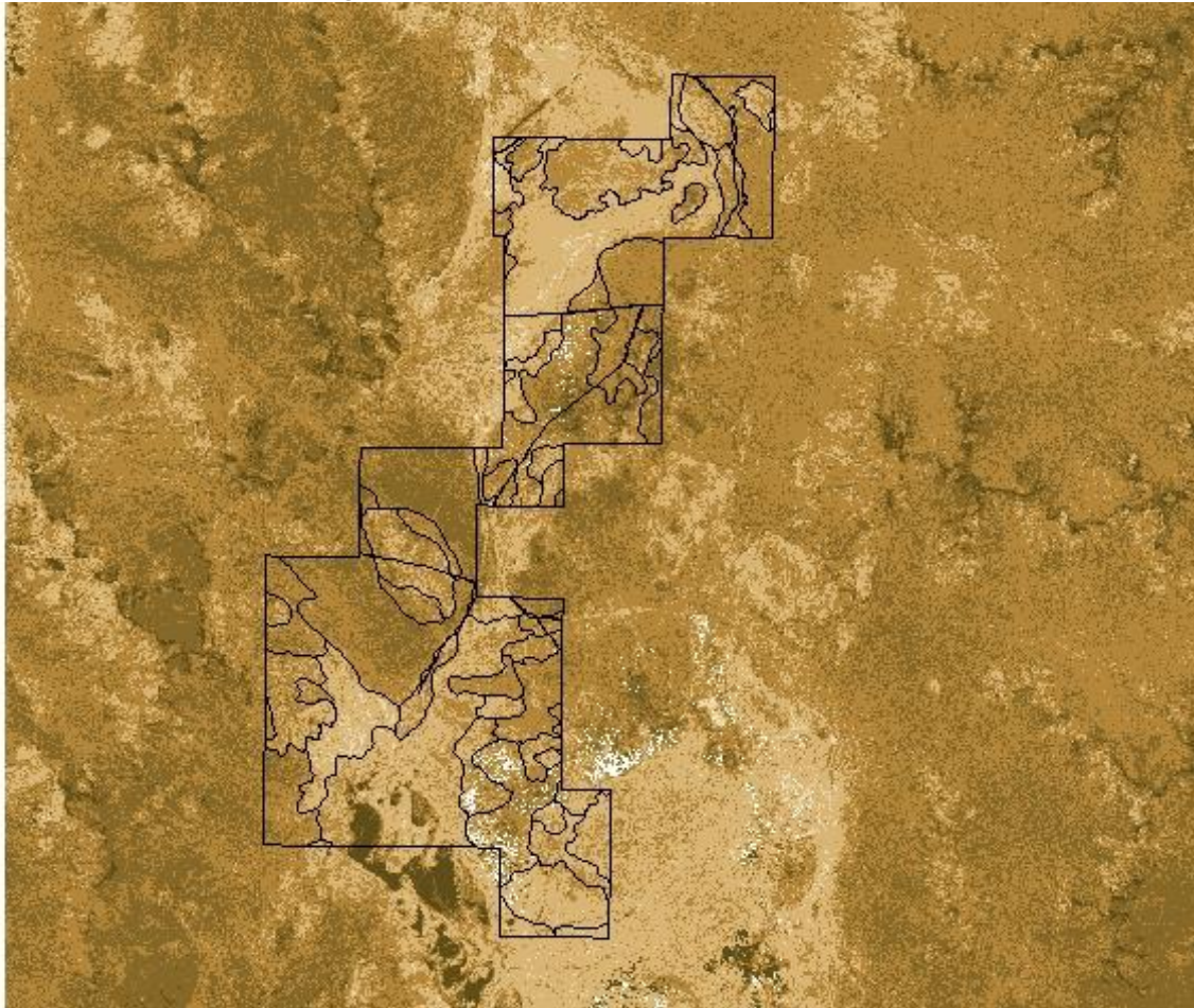
Figure 2 Estimated Total Vegetation Cover Map
