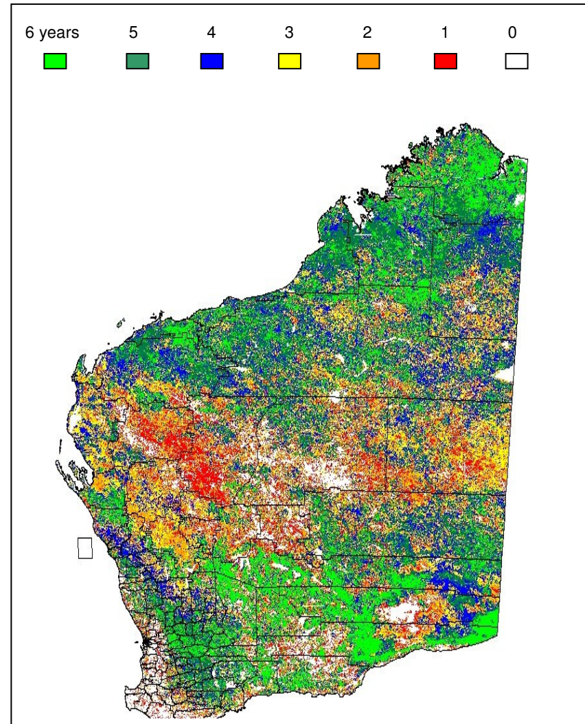
Figure 3. Number of reasonable seasons over the last six years (as determined by NOAA NDVI)
