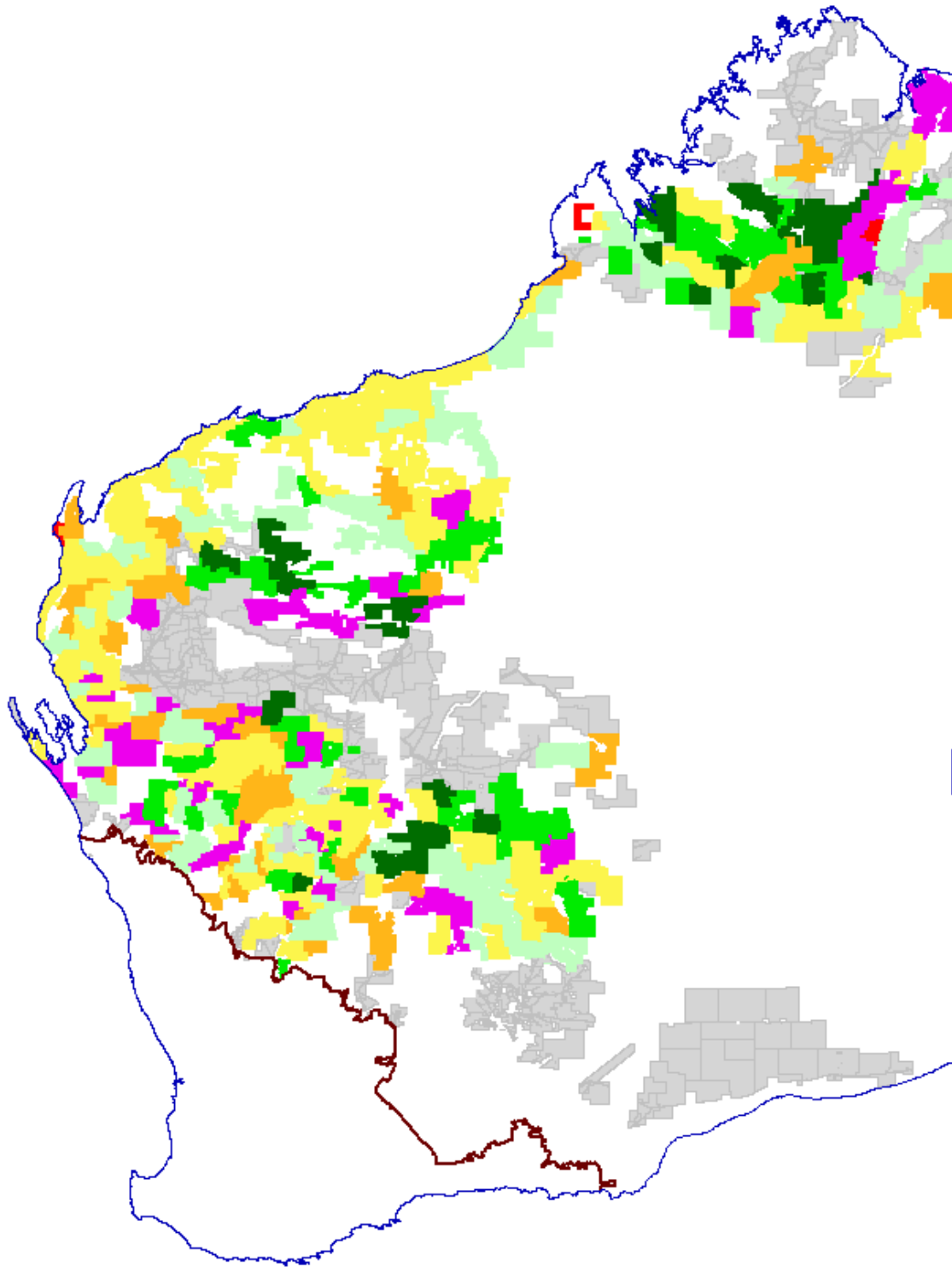
Figure 12. Changes in Range Condition Index between survey (1972 to 2007) and inspection (1999 to 2009)
